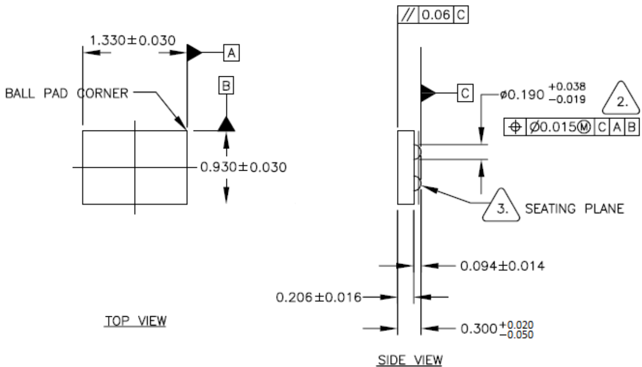
Figure 6 : Package Description (all dimension in mm)
