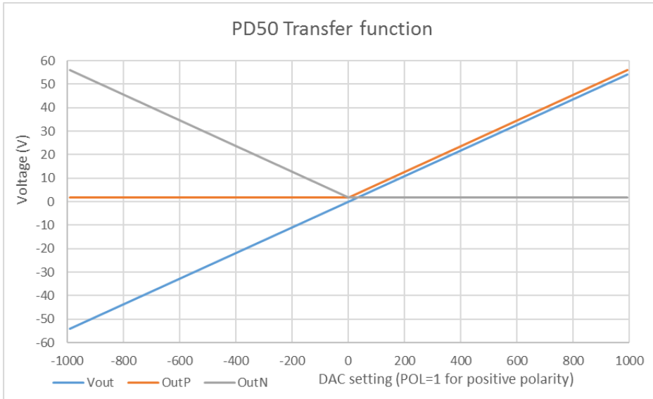
Figure 4 PD50 Transfer function
