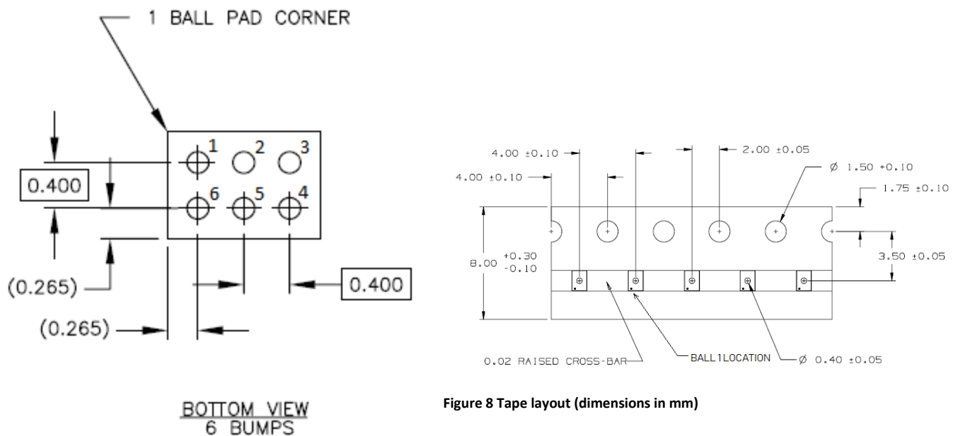
Figure 7 Ball layout (all dimensions in mm)
